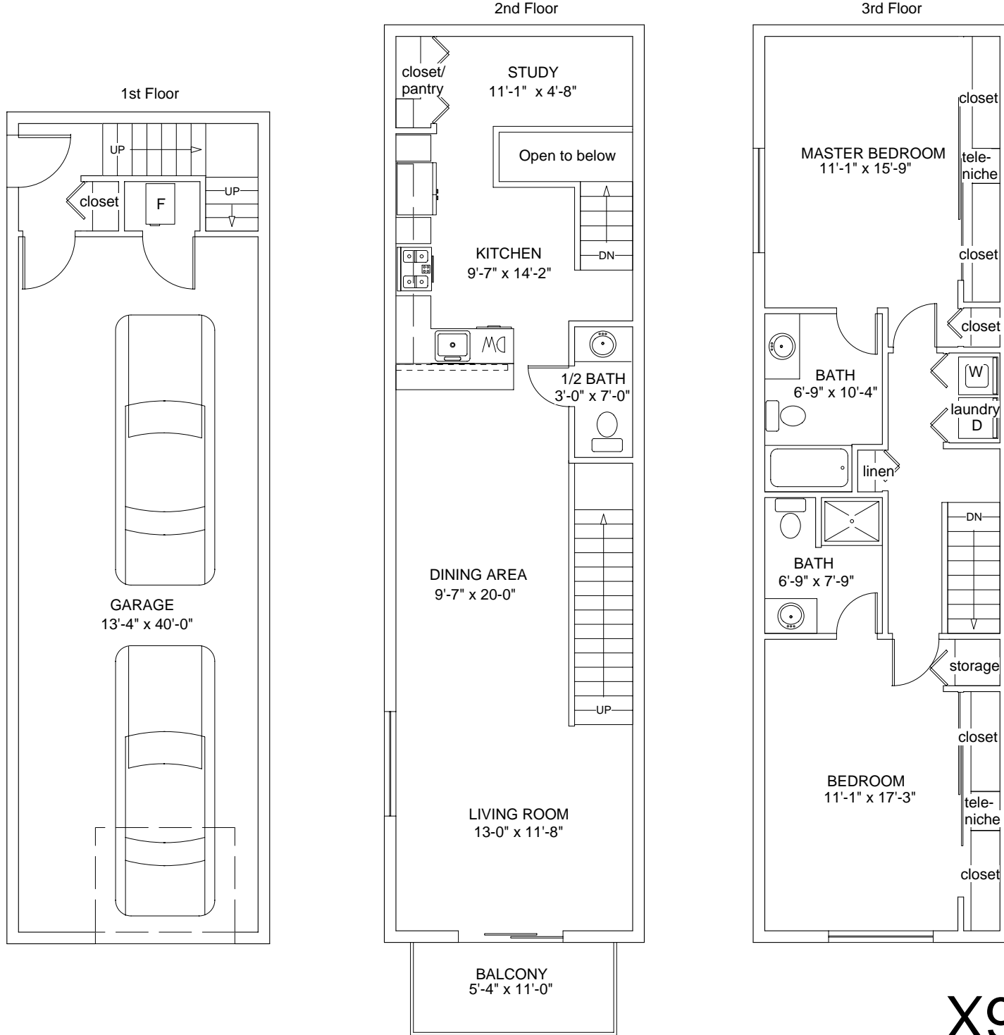
Amber Crossing Townhomes and Lofts 2 Bedroom + Study + 2 1/2 Bath + 2 Car Garage Townhome COLUMBUS 1,290 sq ft + 537 sq ft inside garage # 594
