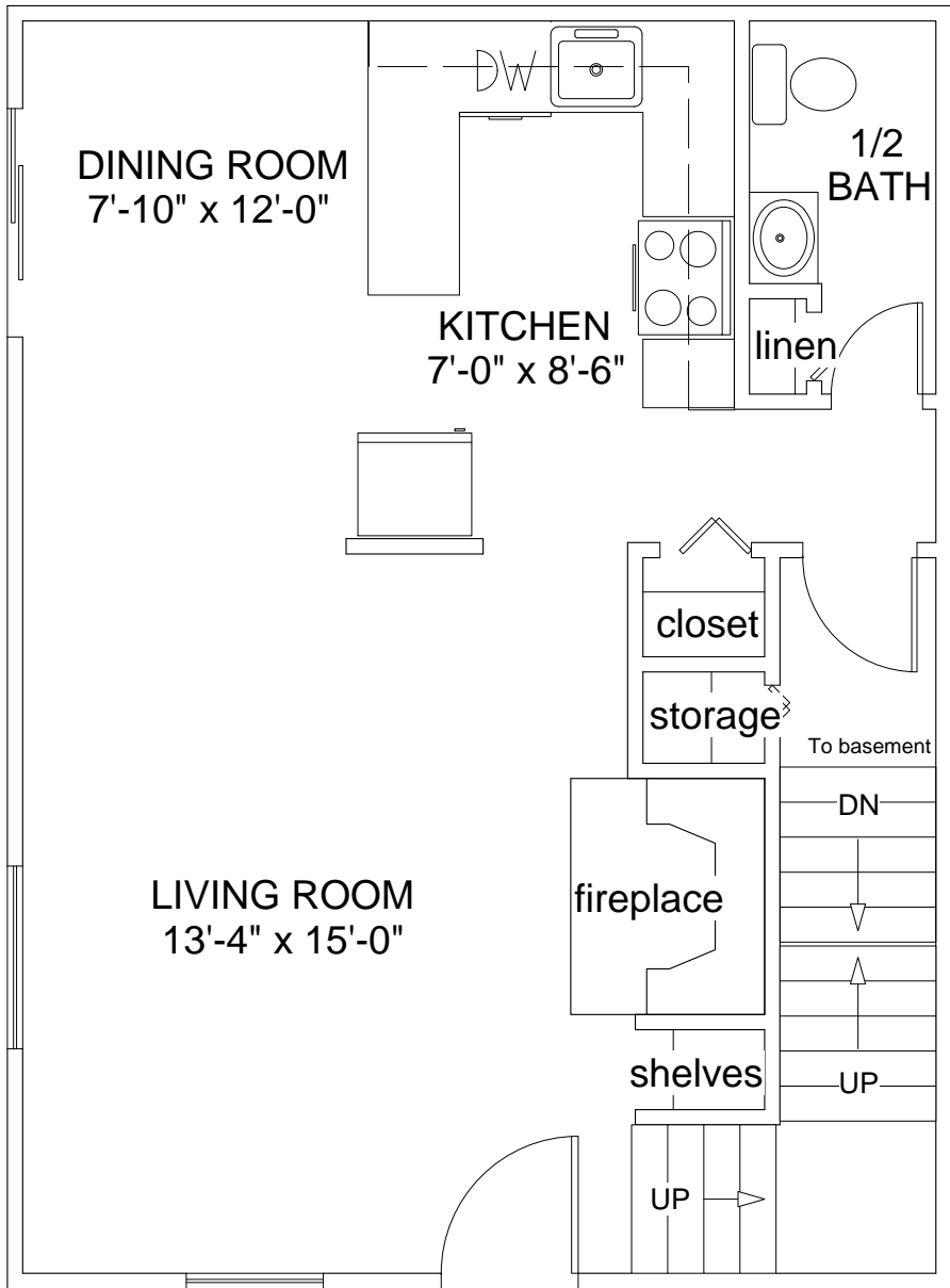
1st Floor
