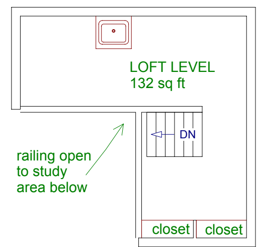
3rd Floor
