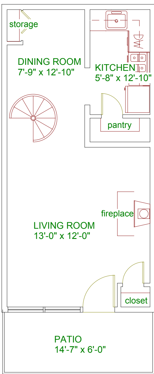
1st Floor
