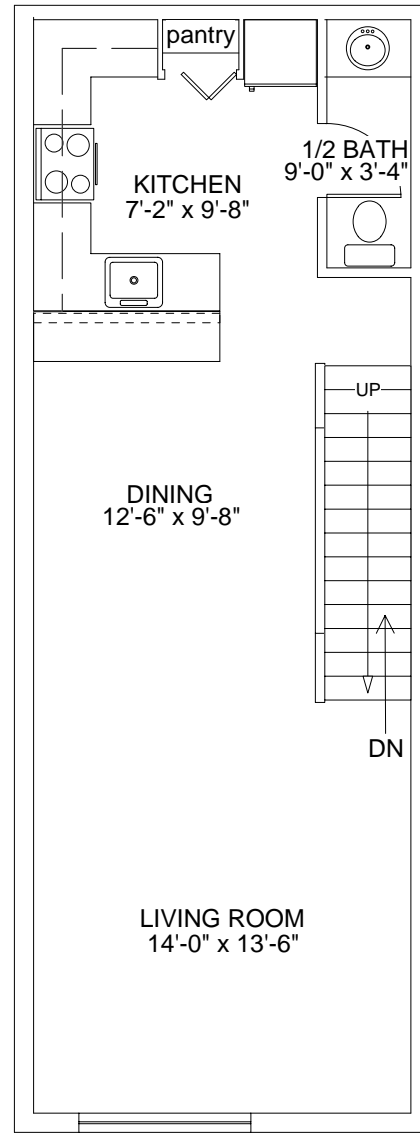
2nd Floor
