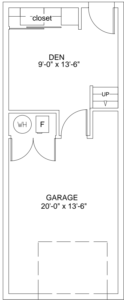
1st Floor
