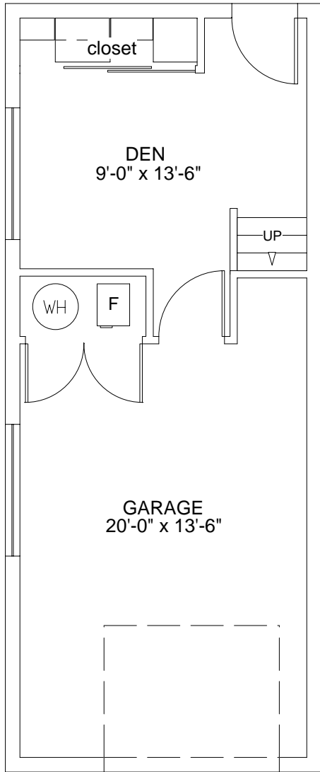
1st Floor
