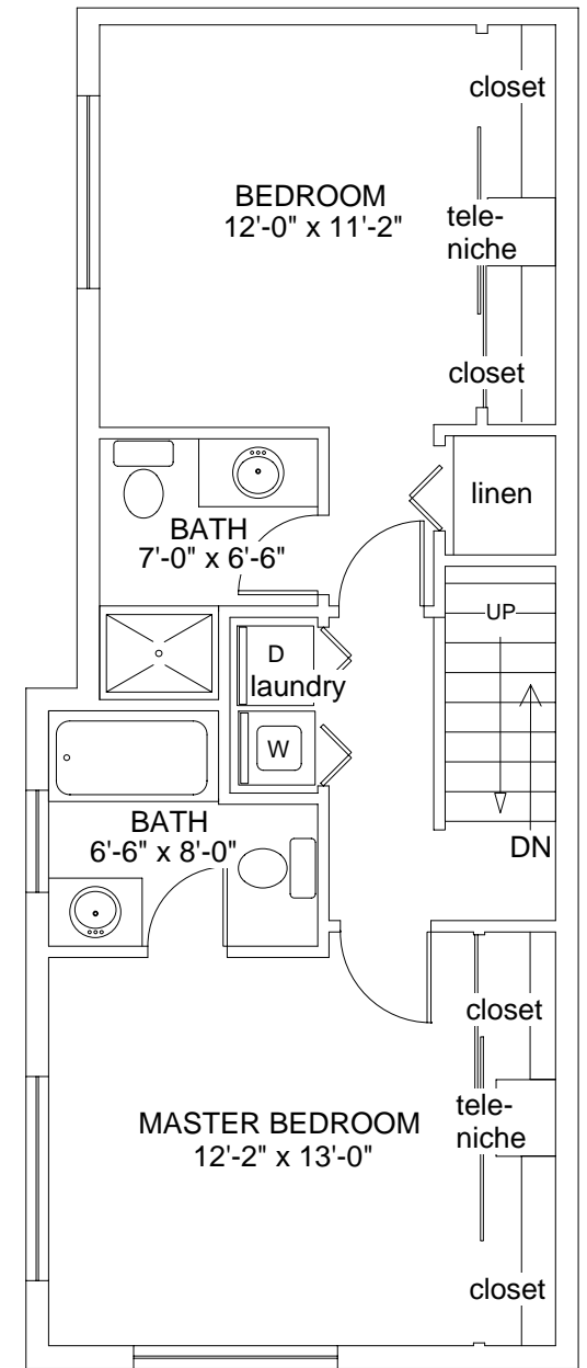
3rd Floor
